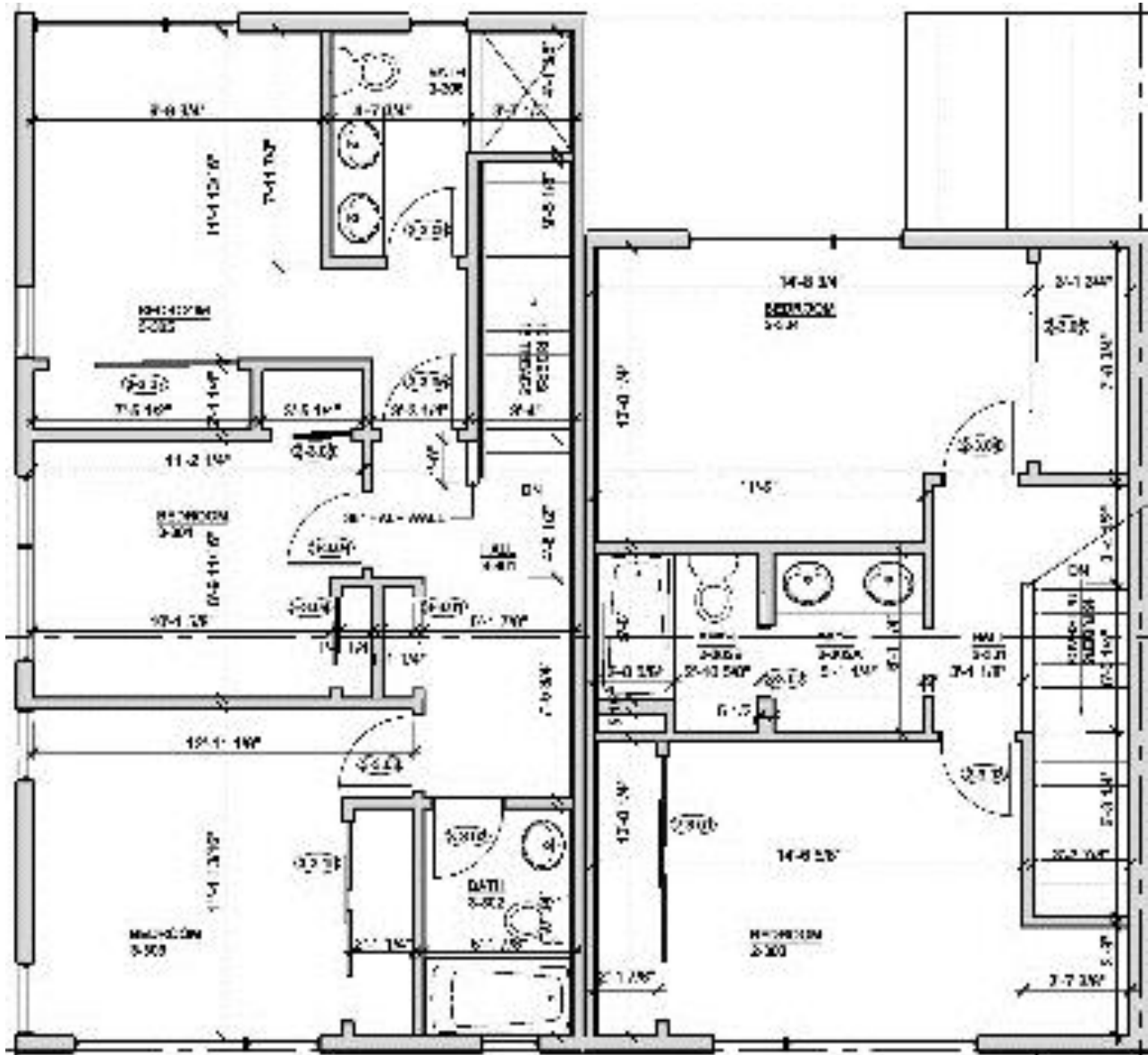
Three Bedroom Unit
